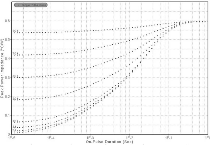
Transient Thermal Response Curve For JCS160N08I(TO-220C)
